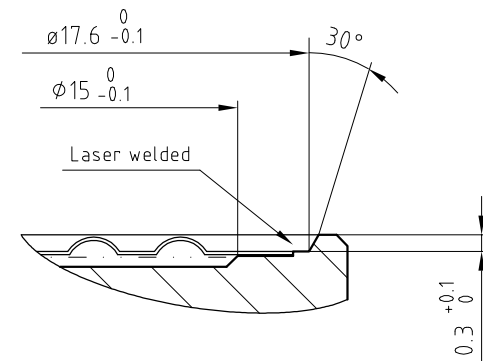
Detail A M10:1
