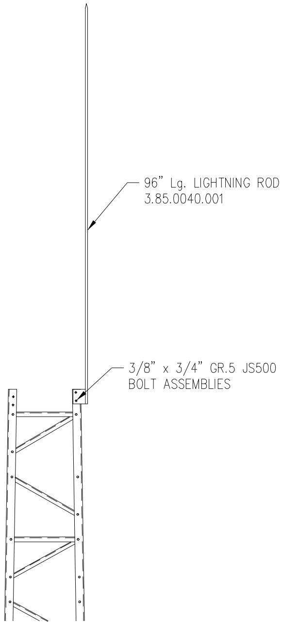
LIGHTNING ROD KIT P/N 4.90.0100.000
