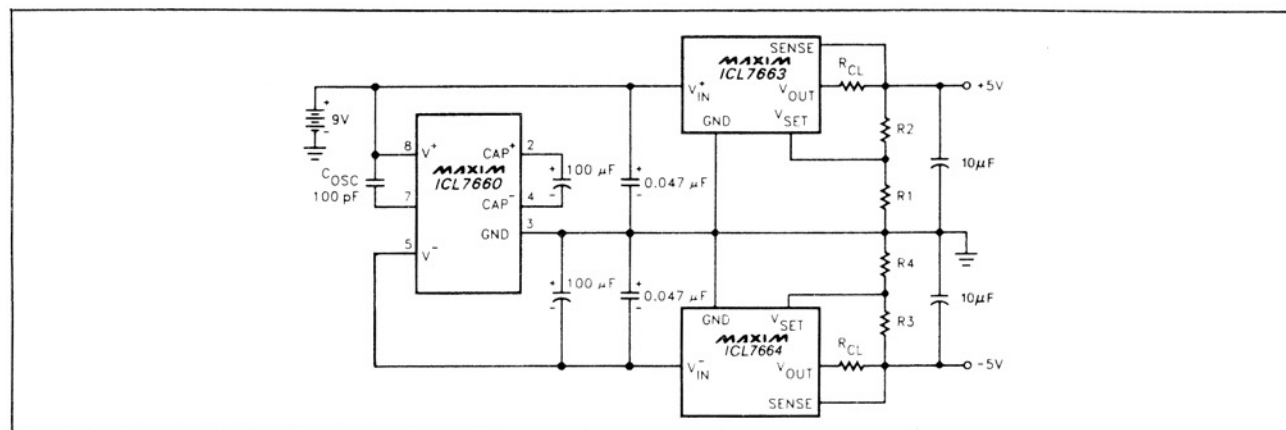
Figure 7. ±5V power supply using one 9V battery.
