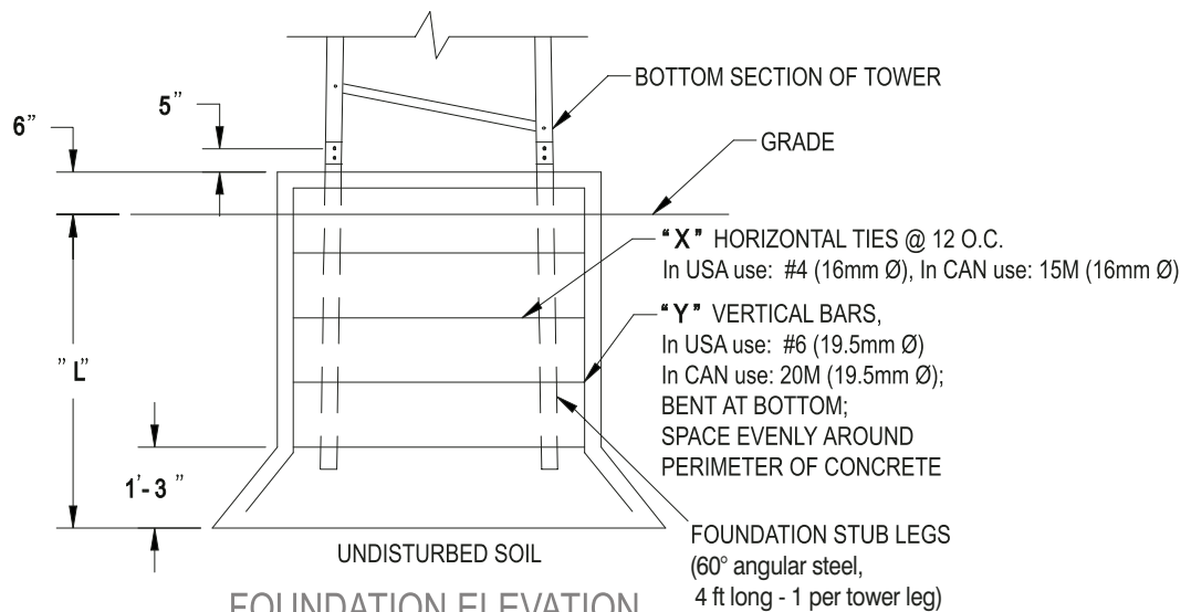
FOUNDATION ELEVATION
